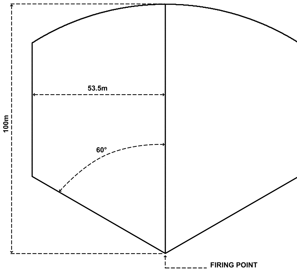
Figure 8-8. 25mm plastic base Sabot discard hazard area
